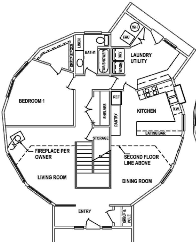
POPLAR - FIRST FLOOR
